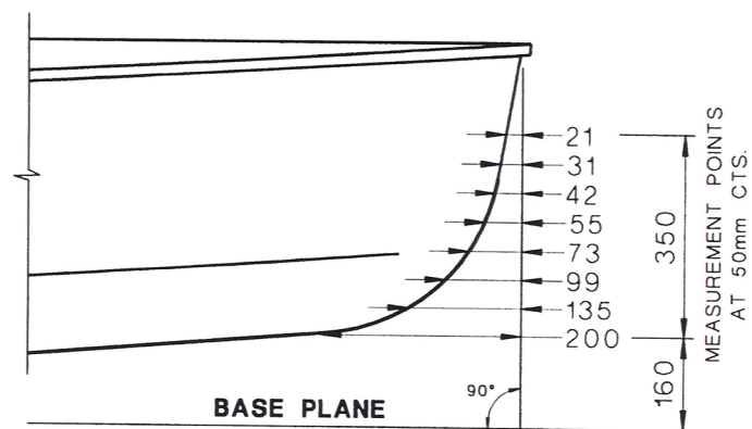
BOW DETAIL
