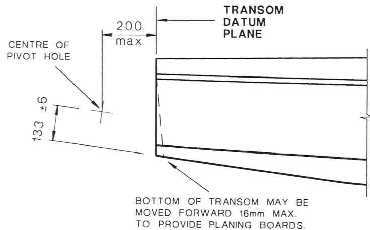
STERN DETAIL
