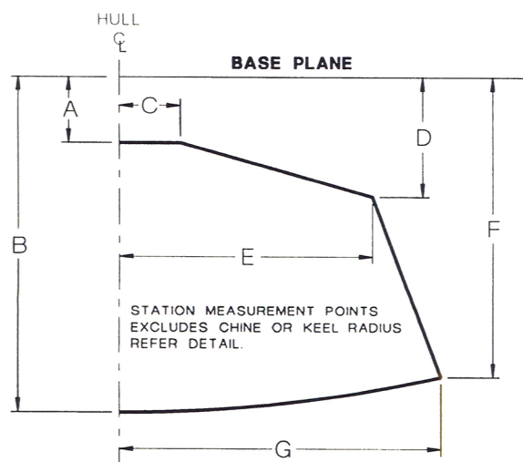
TYPICAL STATION - HALF SECTION
