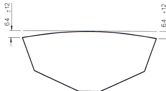
DECK CAMBER CHECK
