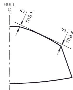
ROUND CHECK STATIONS 0 - 8
