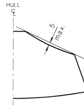
HOLLOW CHECK STATIONS 0 - 8
